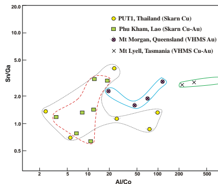
Scatter plot of Al/Co against Sn/Ga by PIXE analyses shows that magnetite samples from the Cu and Cu-Au skarn deposits from Thailand and Laos have a broadly similar Sn/Ga ratio to those from Mt Morgan (Au) and Mt Lyell (Cu-Au) VHMS systems
