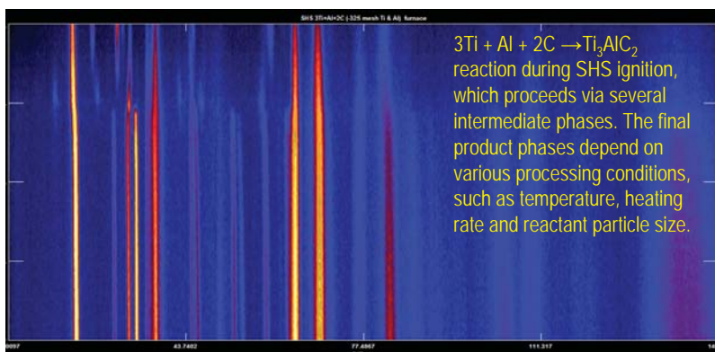
Figure 2 – Time-resolved neutron diffraction of the ignition mechanism during self-propagating high-temperature synthesis (SHS) of titanium aluminium carbide ( Ti_3AlC_2 ).
