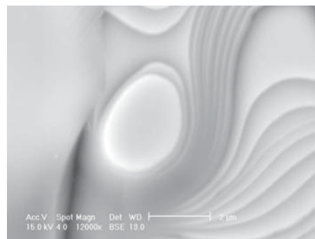
Figure 1 – Scanning electron microscopy (SEM) image of the layered morphology of Ti_3SiC_2 .
