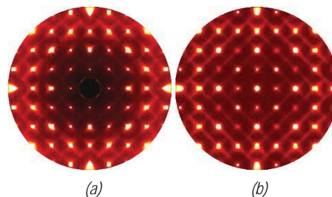
Figure 2: (a) The hk0 plane of neutron diffuse scattering from PZN, measured on SXD at ISIS. (b) The same plane calculated from a model with a domain structure like that seen below.
