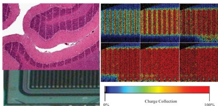
The new dosimeter dimensions (bottom left) will allow probing of the MRT beam (illustrated in the histopathological slide - top left). IBICC images (right) indicate the extent of radiation damage to the new dosimeter.
